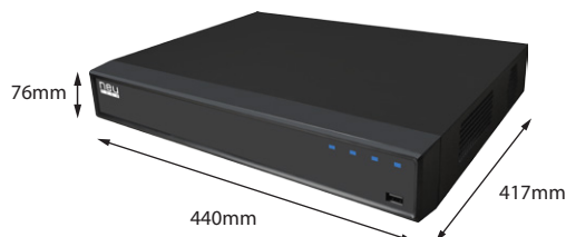
Dimensions (mm)
